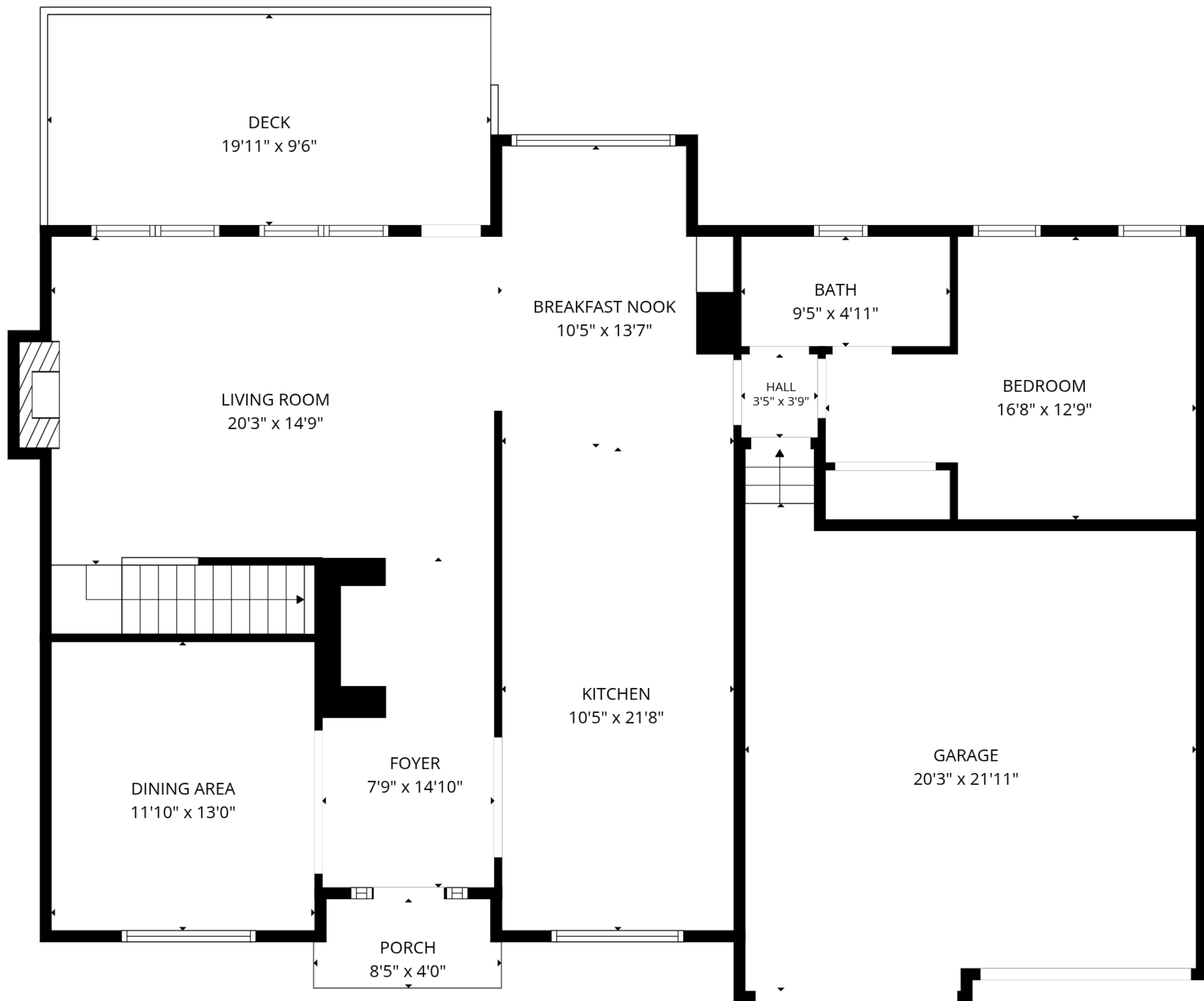
1st floor
